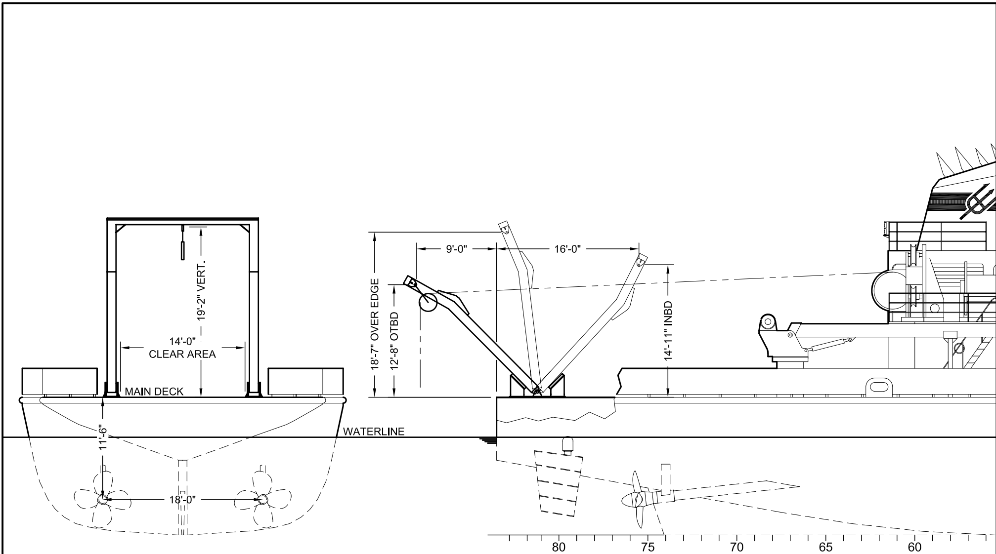
SECTION VIEW VERTICAL A-FRAME POSITION
