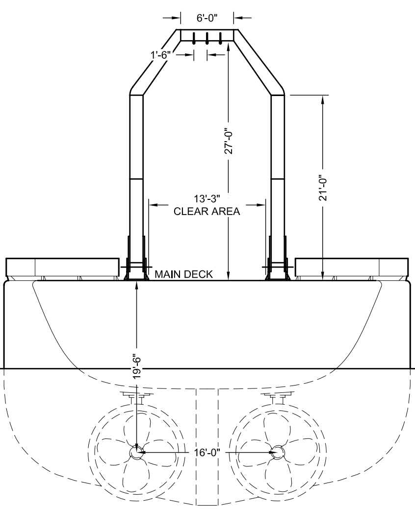
SECTION VIEW VERTICAL A-FRAME POSITION
