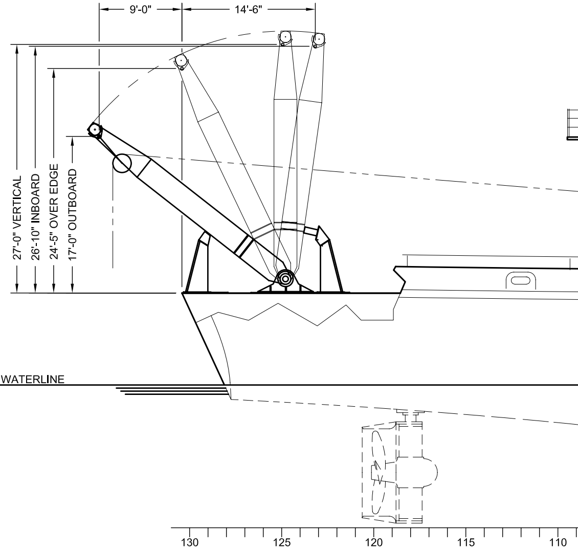
PROFILE VIEW INBOARD/OUTBOARD REACH
