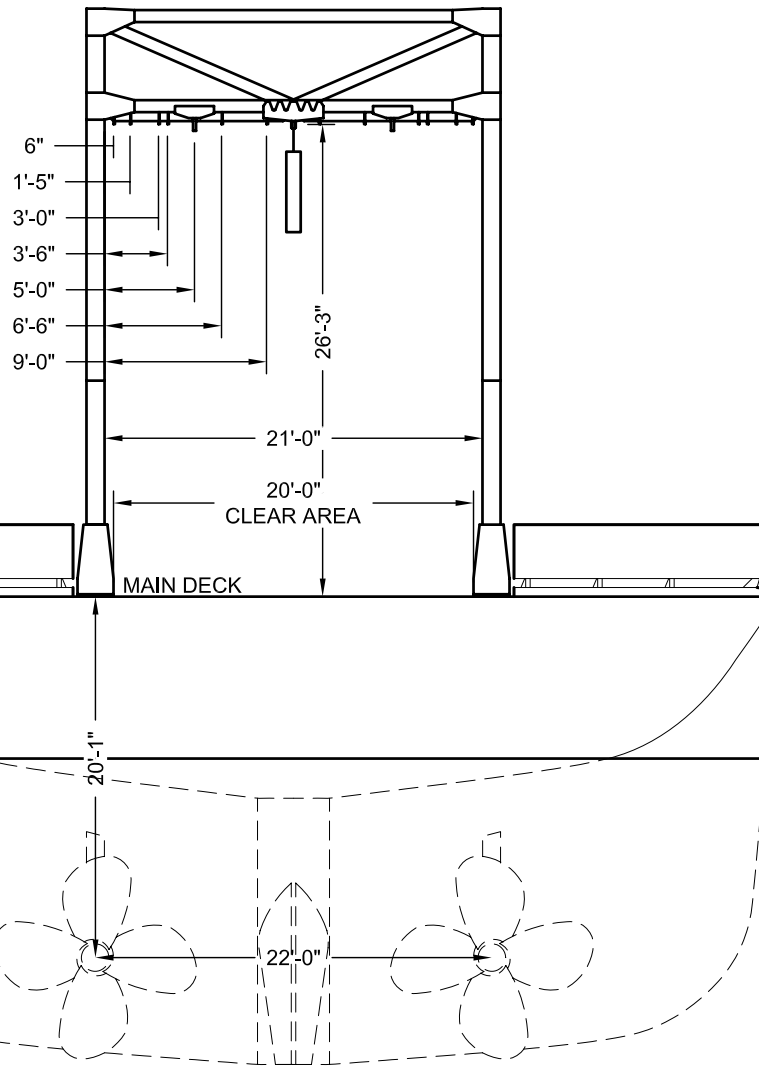
SECTION VIEW VERTICAL A-FRAME POSITION
