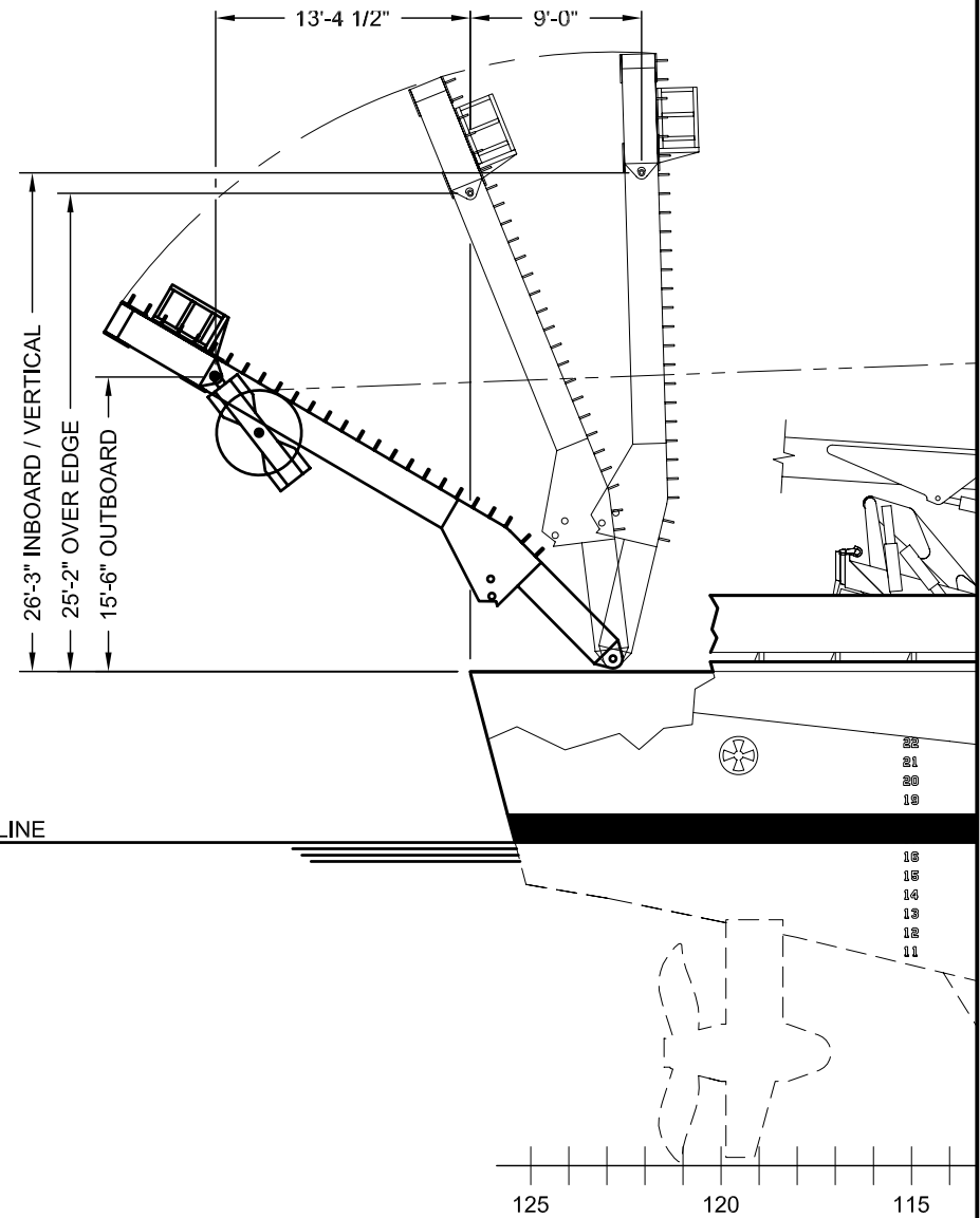
PROFILE VIEW INBOARD/OUTBOARD REACH
