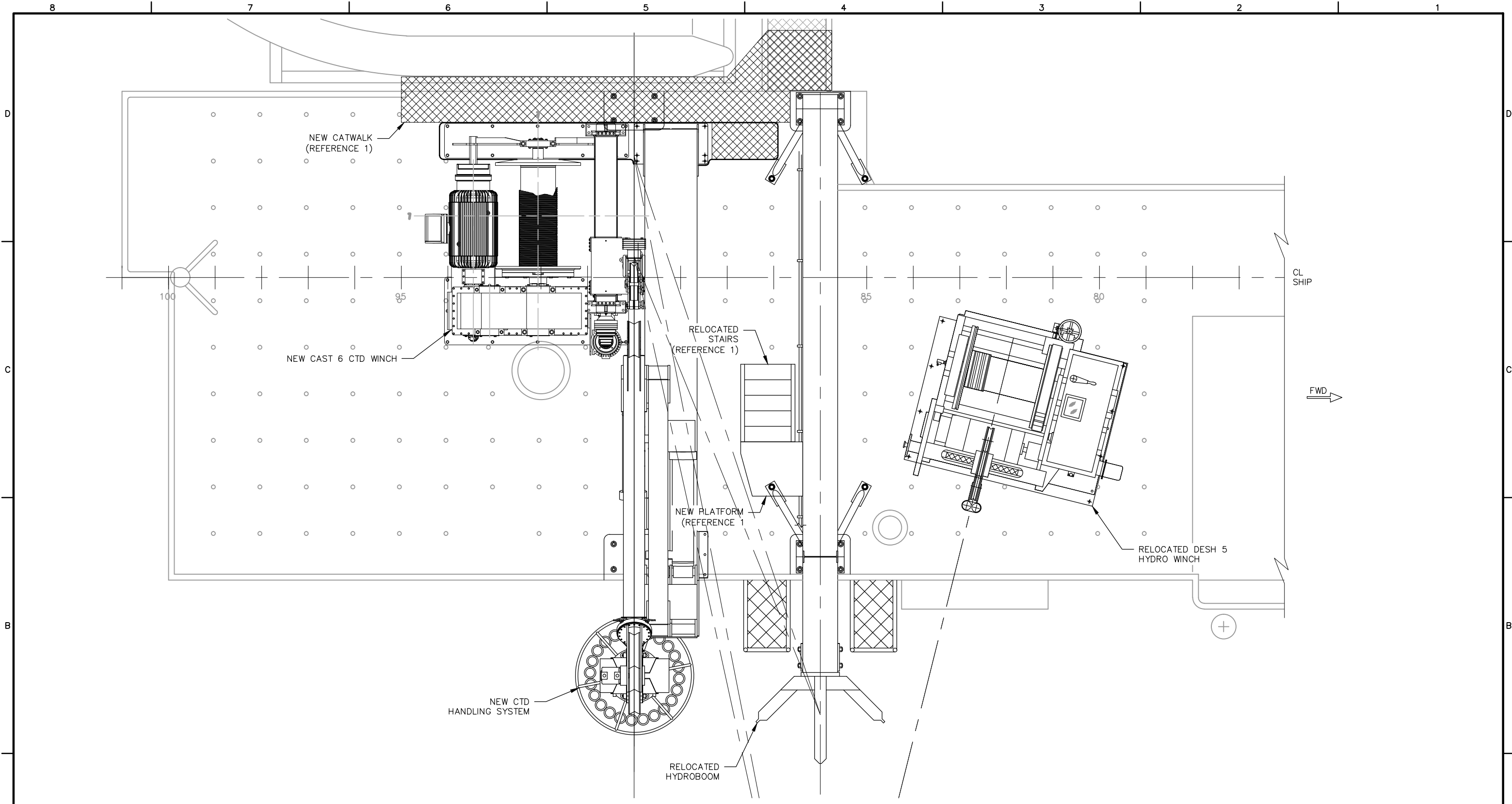
PLAN 3-5A NEW ARRANGEMENT - 02 LEVEL 1/4" = 1'-0"
