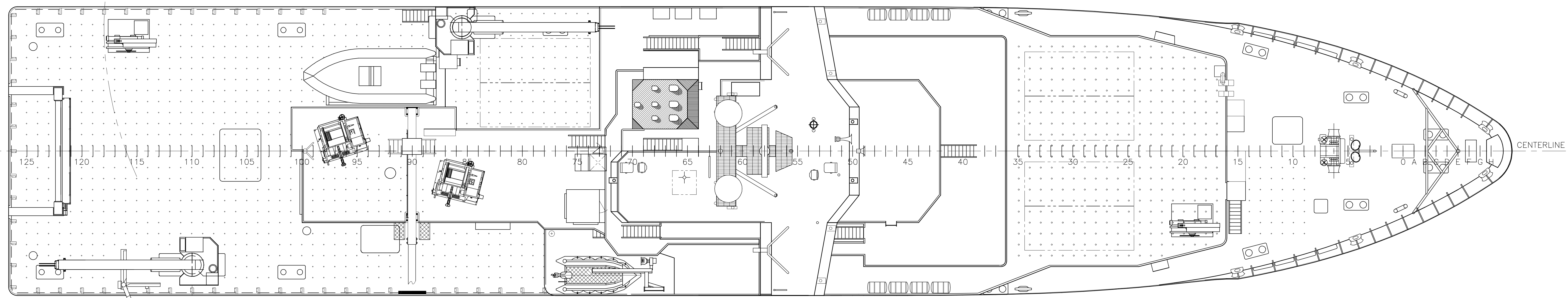
R/V REVELLE TOPSIDE CONFIGURATION 3/27/01
